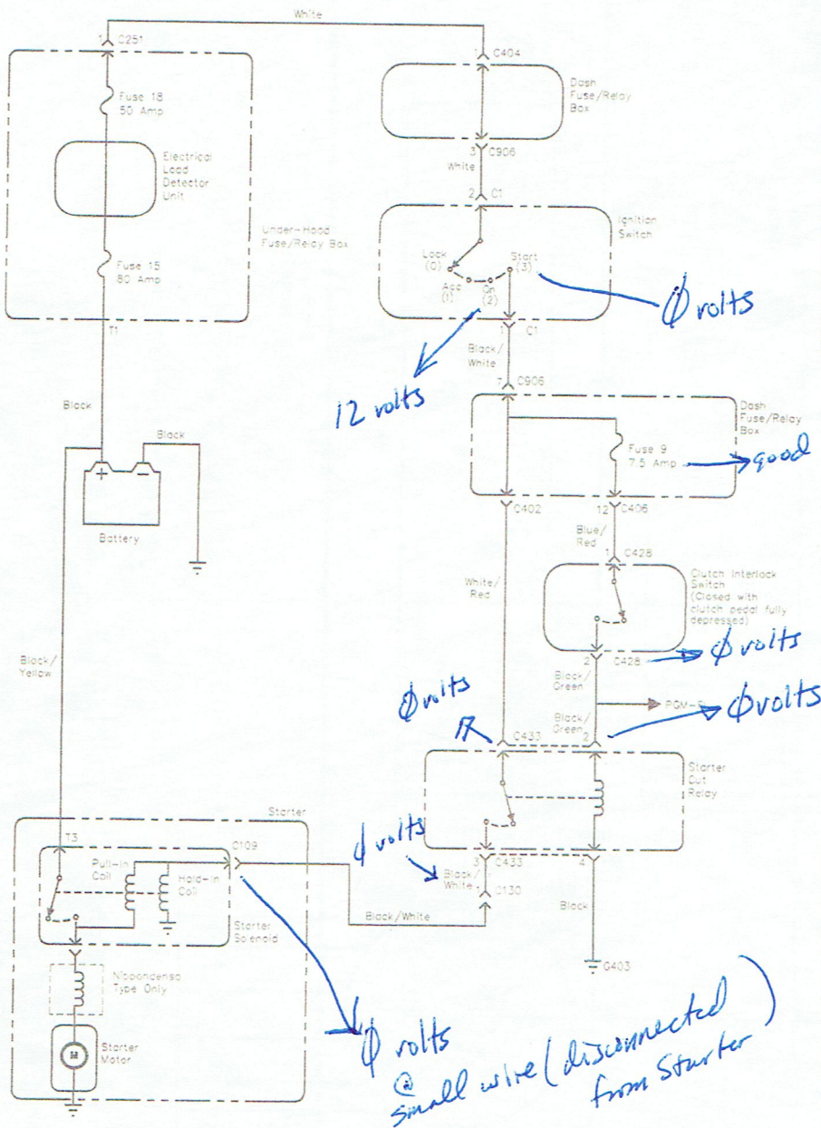
Typical starting system circuit (manual transaxle models)
