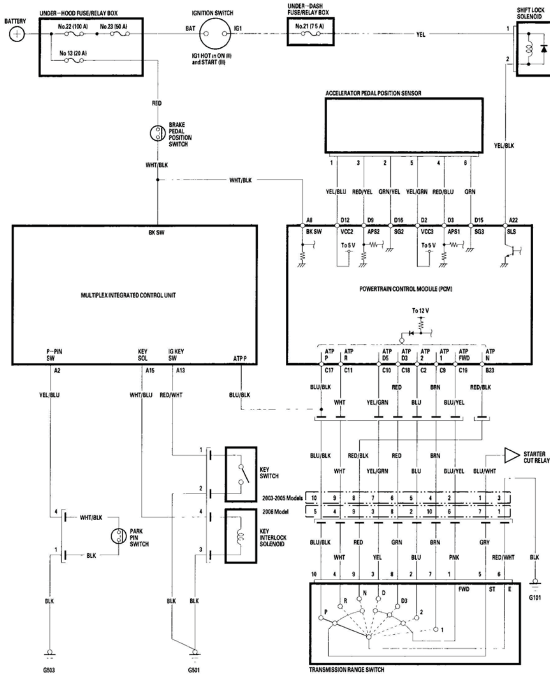
Fig. 327: A/T Interlock Circuit Diagram Courtesy of AMERICAN HONDA MOTOR CO., INC.
